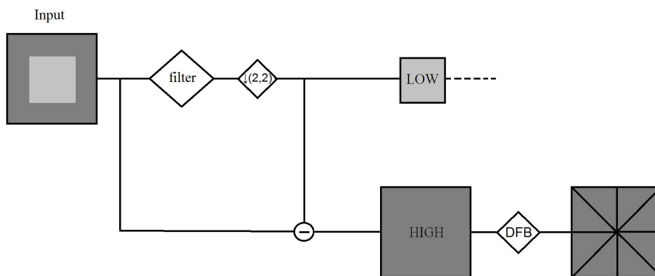
Figure 1. The Contourlet Filter Bank.
